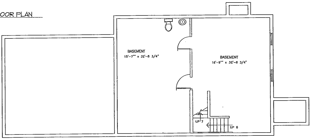
BASEMENT/FOUNDATION PLAN 1/4" = 1'-0"
