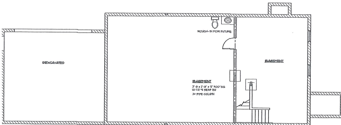
BASEMENT PLAN 1/4" = 1'-0"
