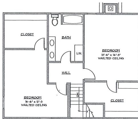
SECOND FLOOR PLAN 1/4" = 1'-0"
